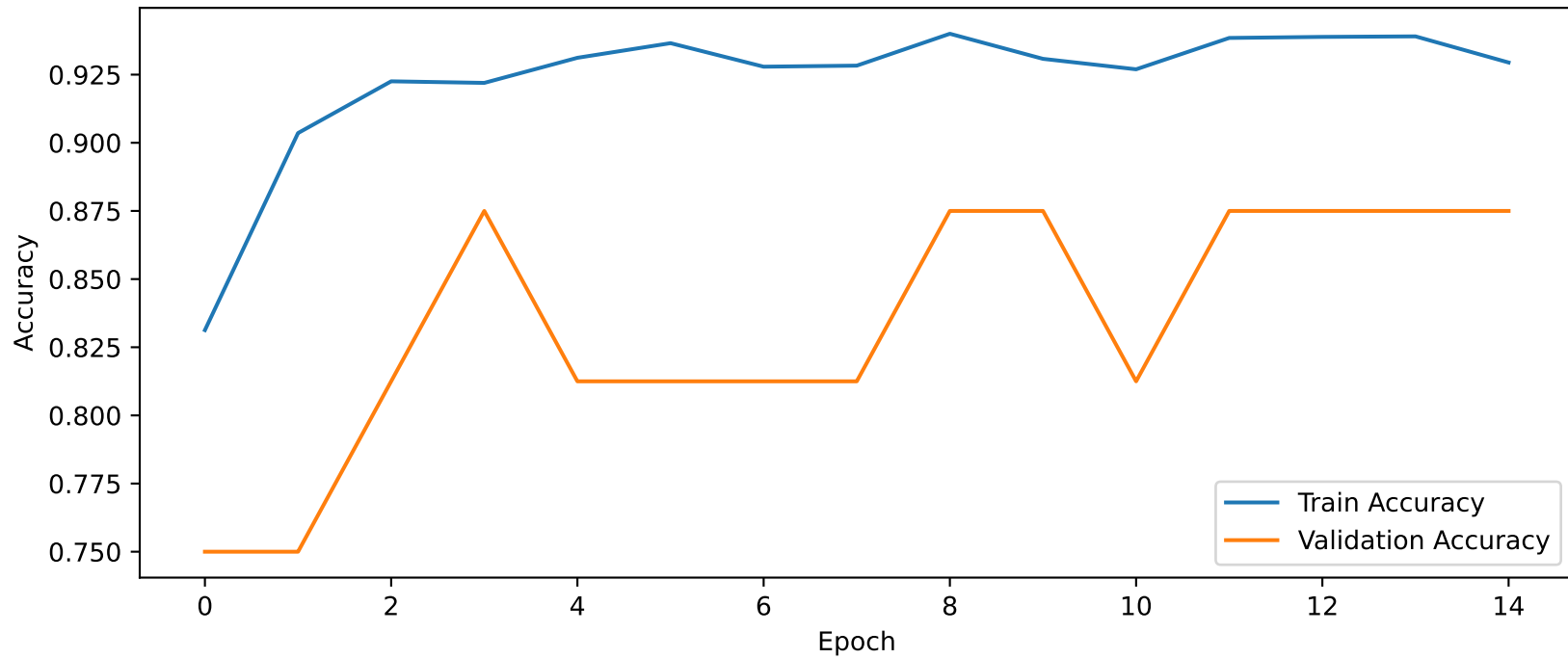
Training vs Validation Accuracy Frozen Feature Extractor
