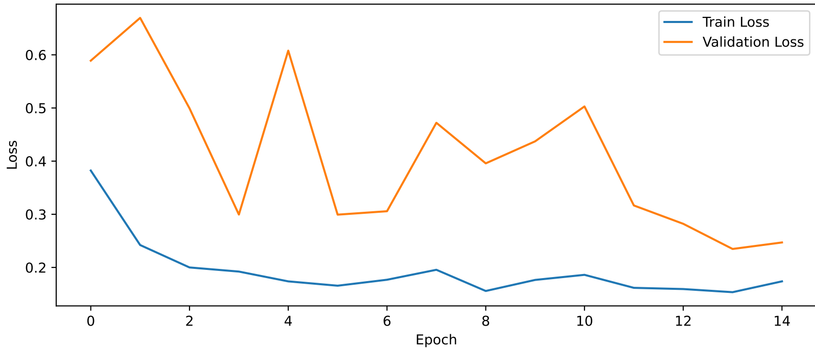
Training vs Validation Loss Frozen Feature Extractor
